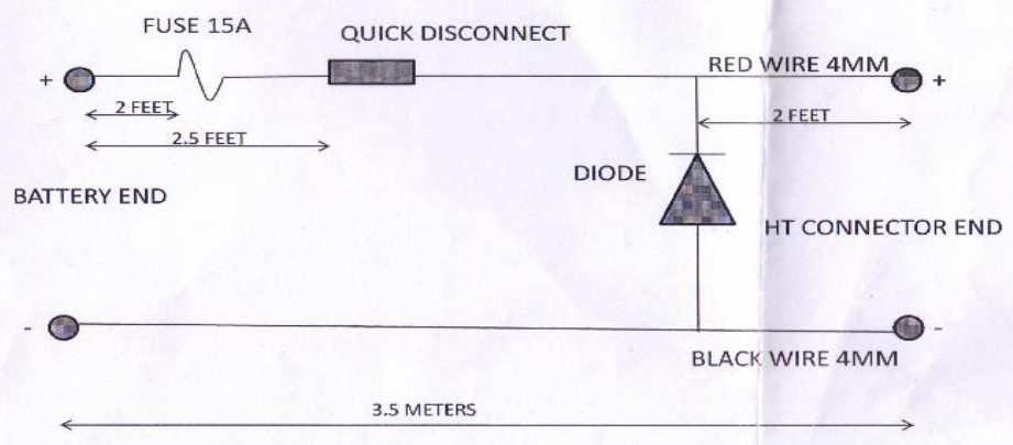
DIAGRAM OF LT LEAD FOR GM 300/338/950 WT SETS
